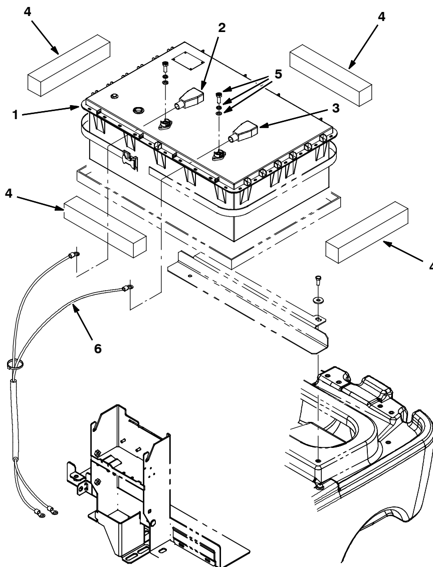
Fig. 8 - Battery Group, 160Ah, Lithium-Ion (China)
