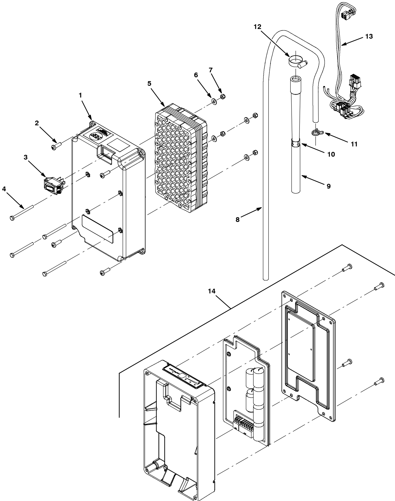
Fig. 3 - ec-H2O NanoClean Module Breakdown, 9011810 (S/N 30044871- )
