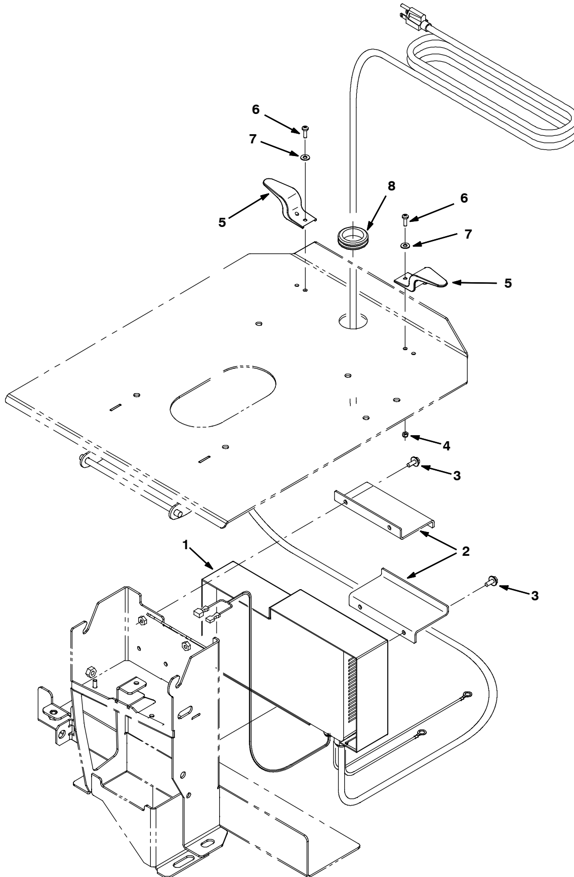
Fig. 13 - Battery Charger Kit, On-Board (S/N 30044871- )
