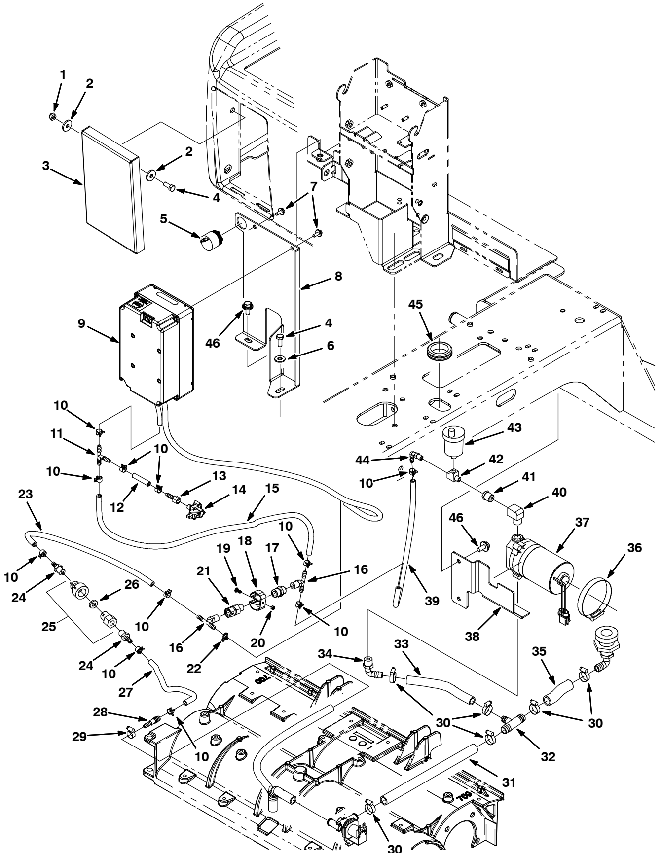
Fig. 6 - ec-H2O Group, Cylindrical Scrub Head (S/N 30000000-30044870)
