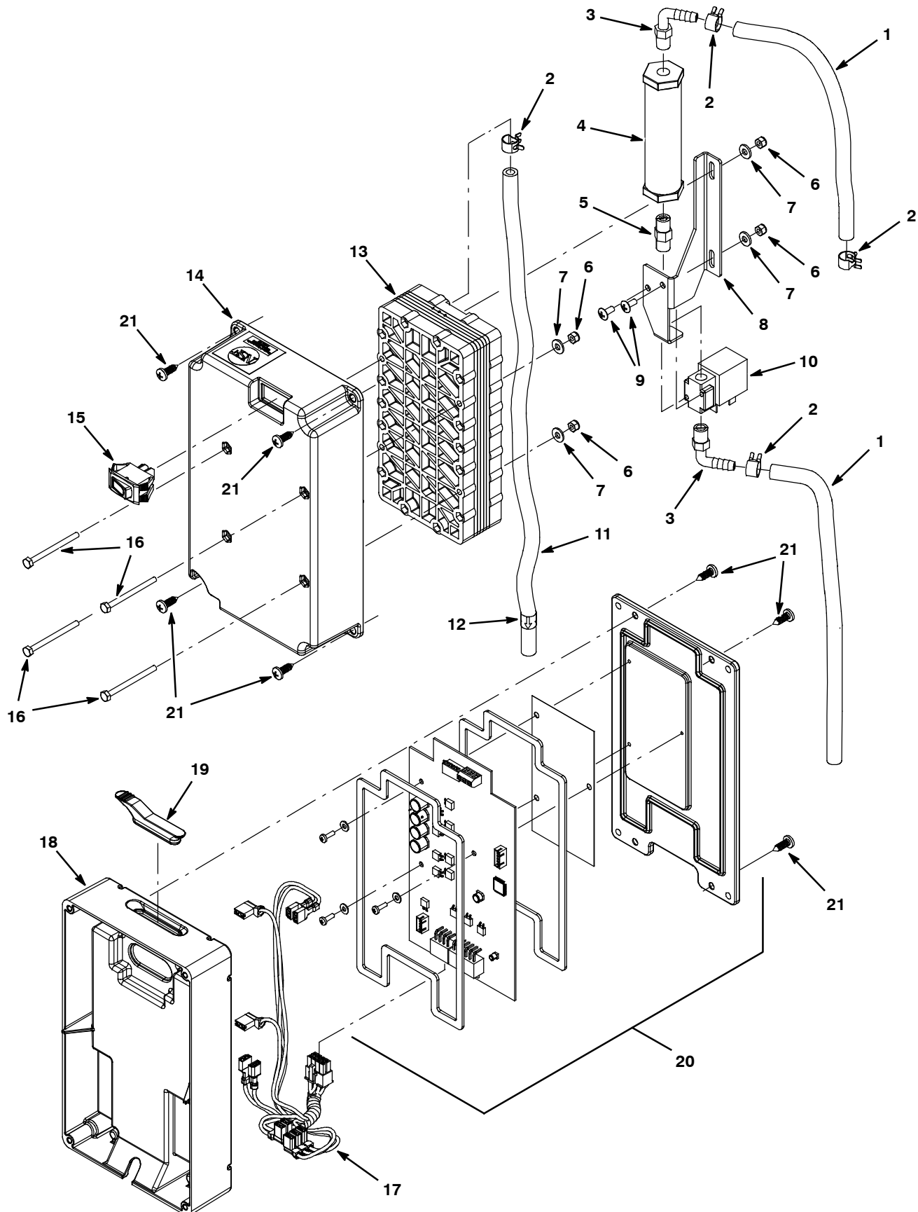
Fig. 4 - ec-H2O Module Assembly Breakdown, 9007970 (S/N 30000000-30044870)
