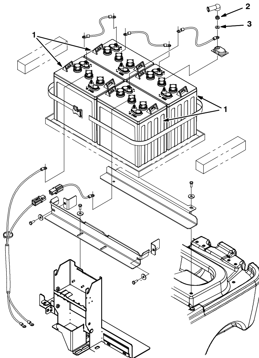
Fig. 9 - Battery Group, 260Ah (China)
