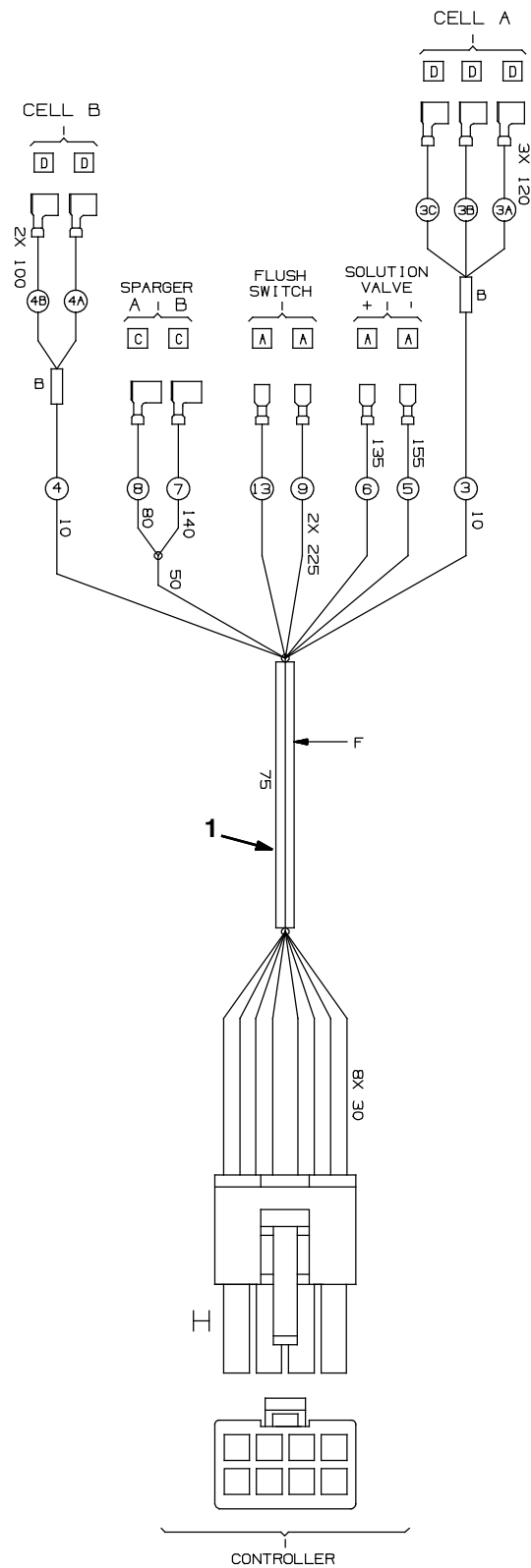
Fig. 43 - Wire Harnesses Group, ec-H2O Main Control Board (S/N 30000000-30044870)
