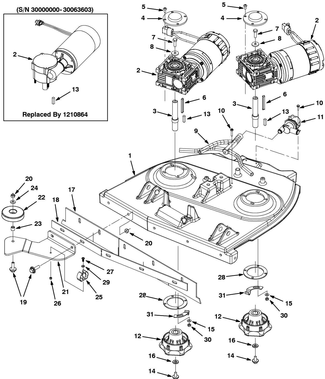
Fig. 13 - Disk Scrub Head Drive Motor Group, 650 mm (26 in)
