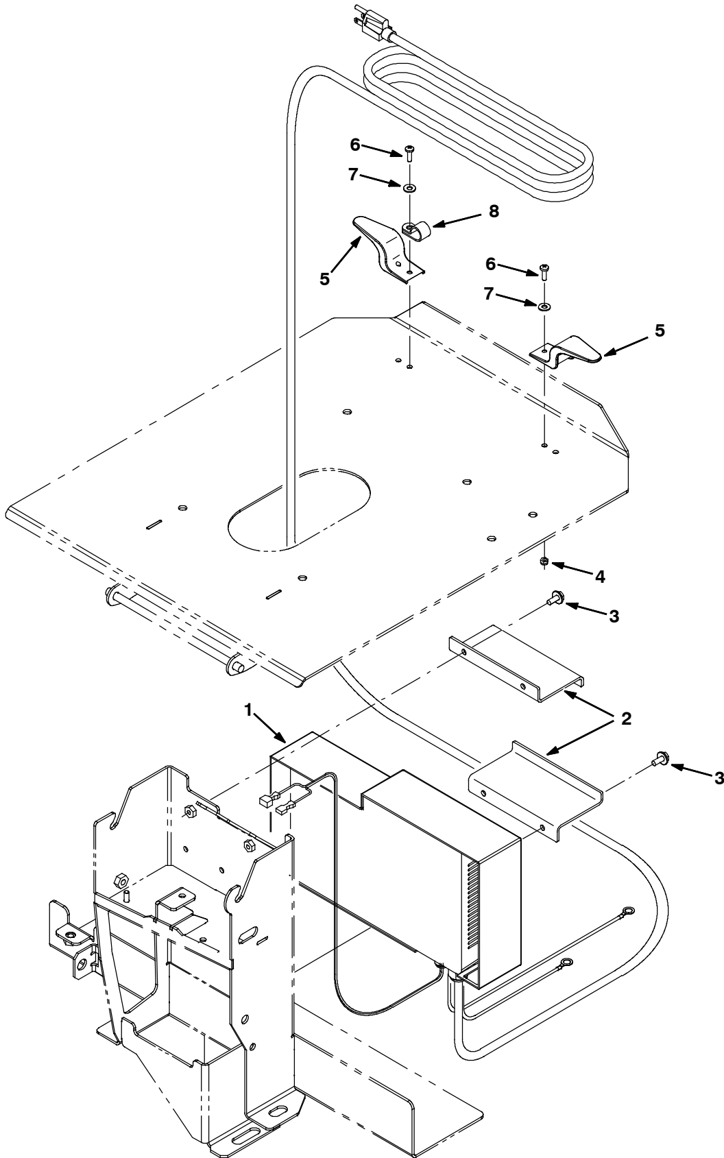
Fig. 14 - Battery Charger Kit, On-Board (S/N 30000000-30044870)
