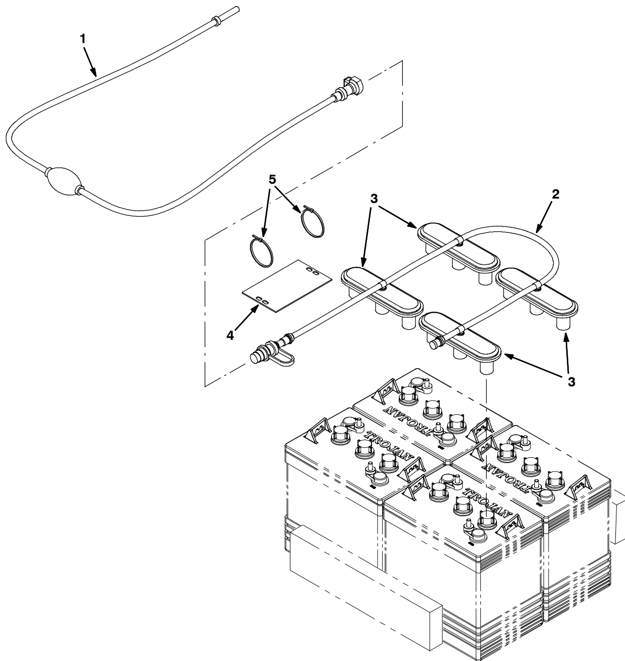
Fig. 16 - HydroLink® Battery Watering System Kit
