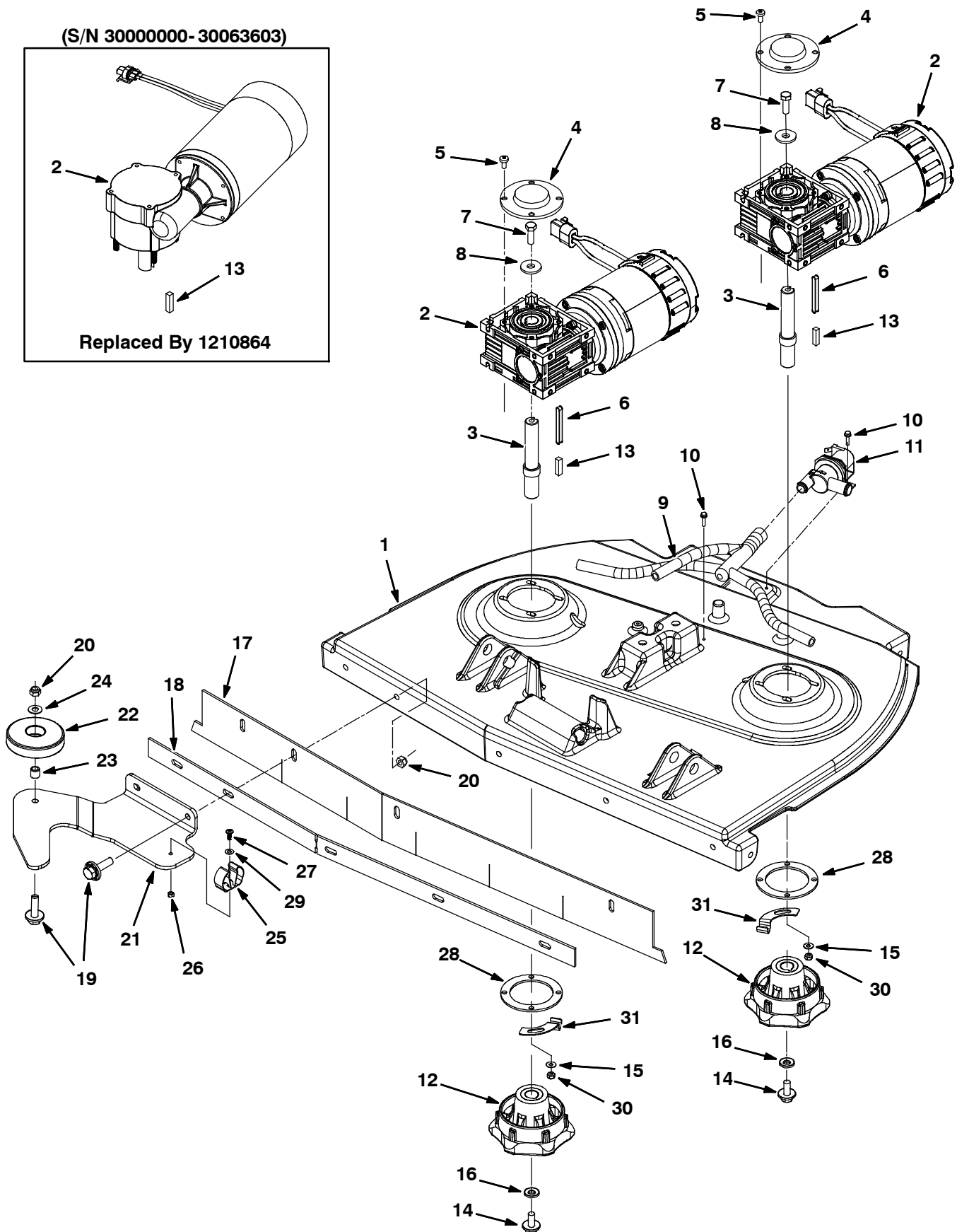
Fig. 14 - Disk Scrub Head Drive Motor Group, 800 mm (32 in)
