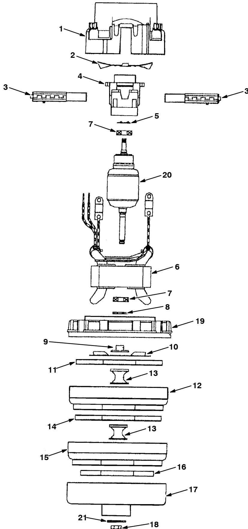
Fig. 6 - Vacuum Fan Motor Breakdown, 1021064
