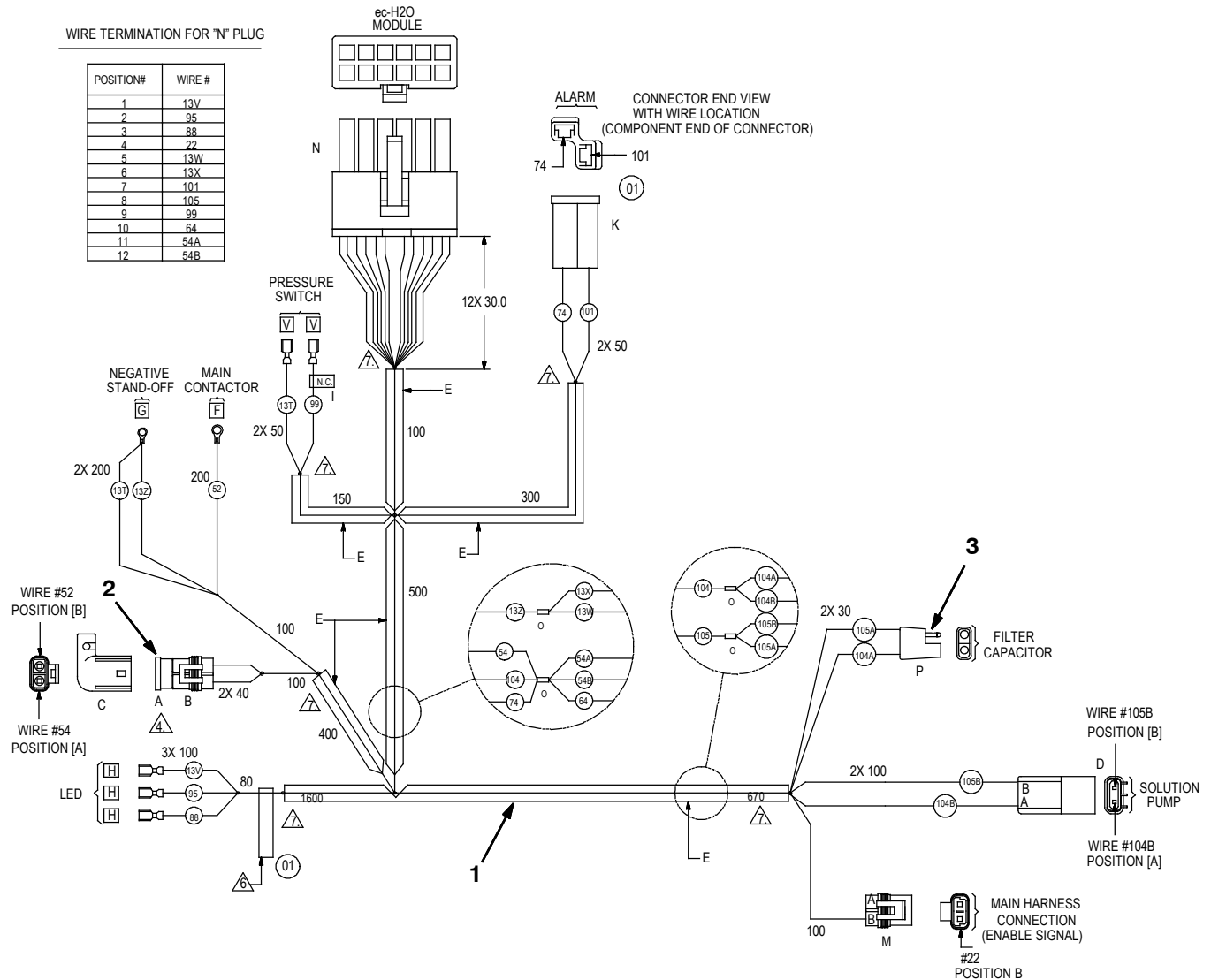
Fig. 41 - Wire Harnesses Group, ec-H2O (S/N 30000000-30044870)
