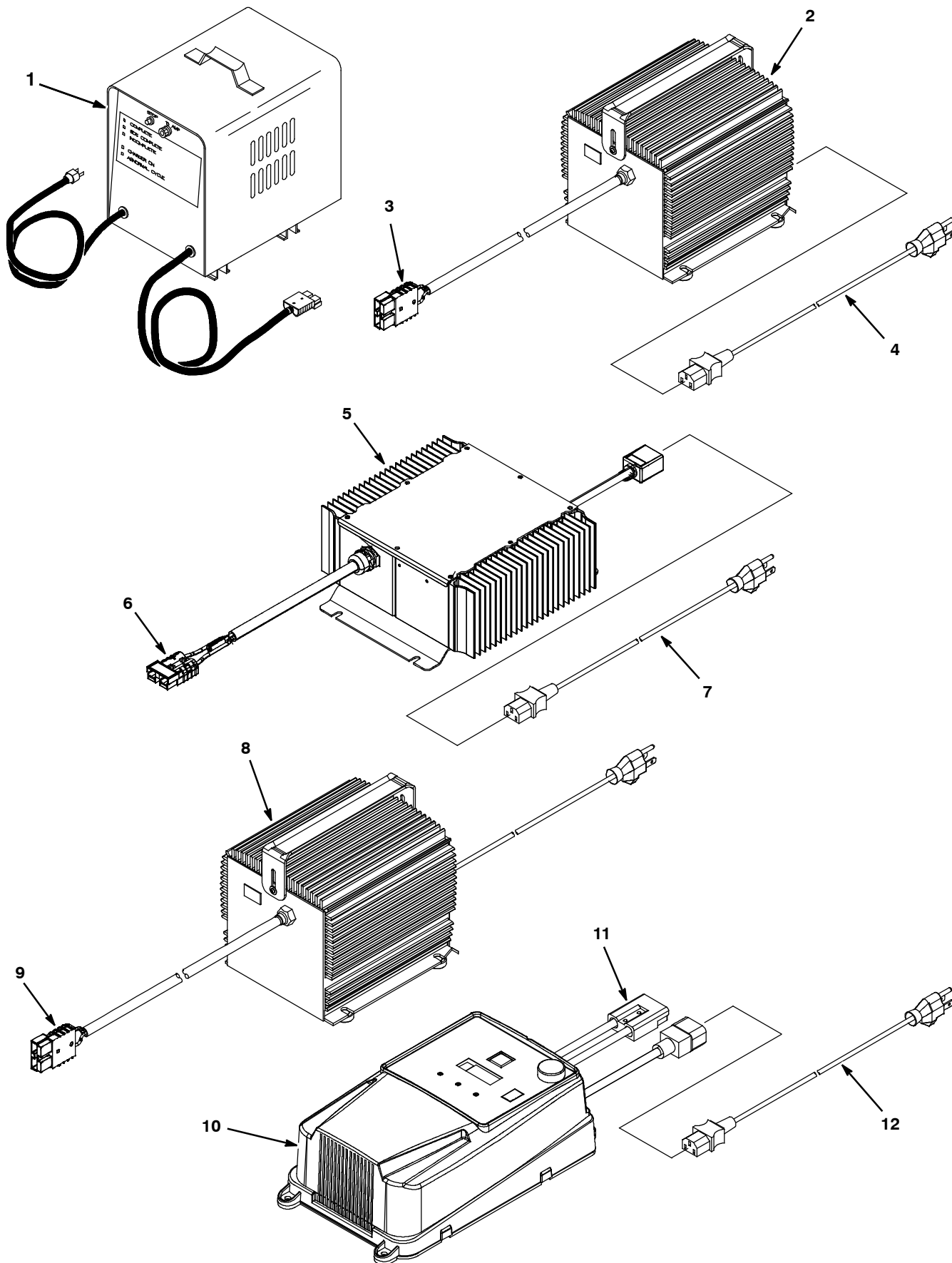
Fig. 15 - Battery Chargers Group, Off-Board
