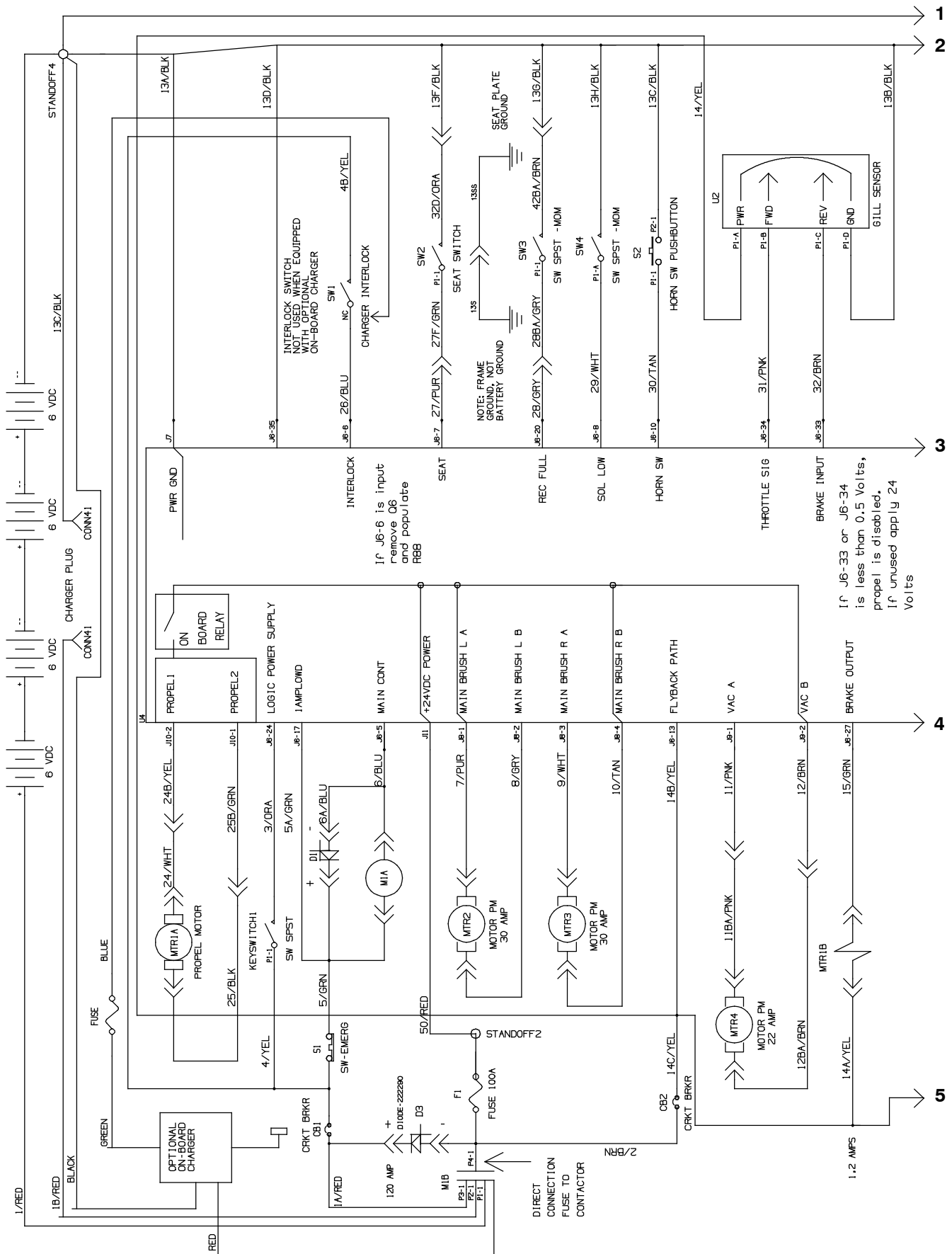
Fig. 36 - Electrical Schematic, Standard & FaST Model (S/N 30000000- 30044870)
